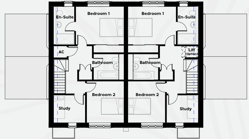
FIRST FLOOR
